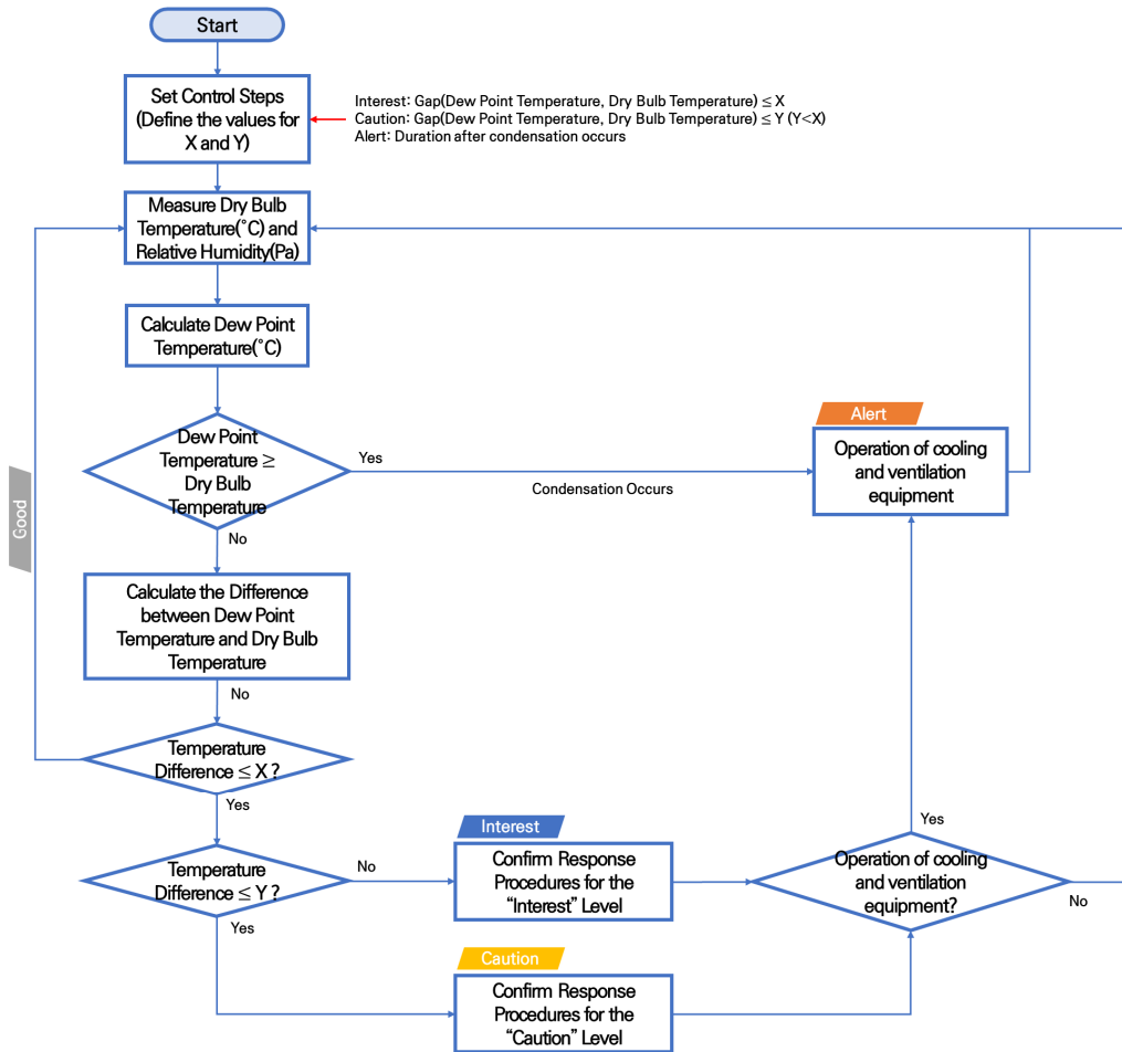
Fig. 2. Flowchart for condensation prediction algorithm using temperature and humidity
