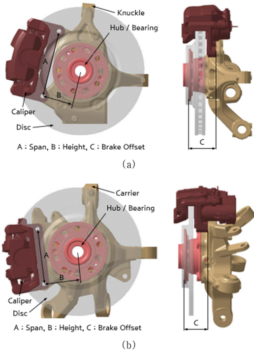
Fig. 1 Modular design of (a) front and (b) rear brake system for medium and large EV
