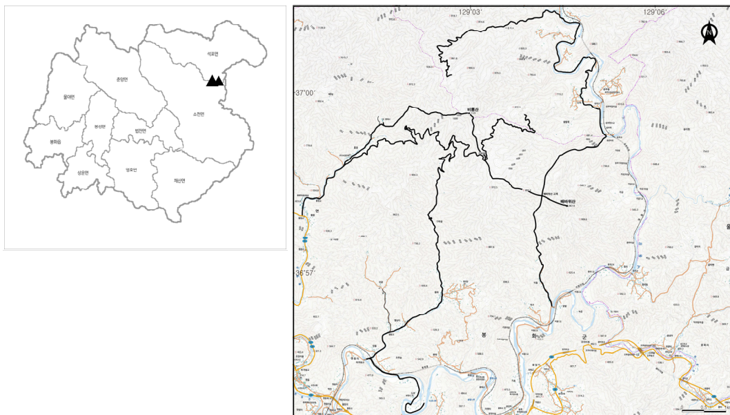
Fig. 1. The survey routes of Biryongsan Mt. and Baebawhisan Mt. (— : survey route).
