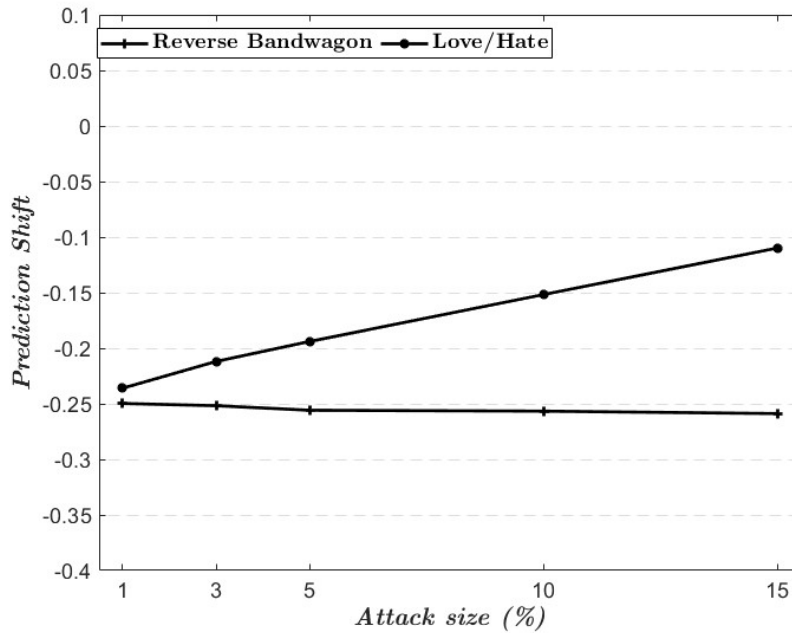
Fig. 6. Prediction shift for different sizes of attack (in nuke attack models)
