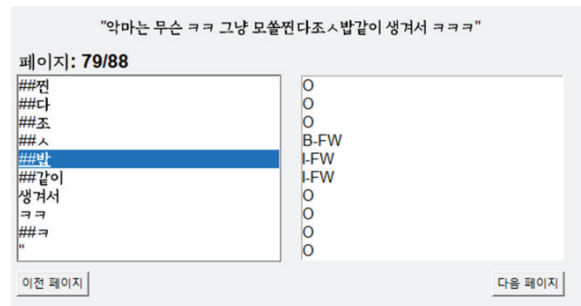
Fig. 1. GUI Program
