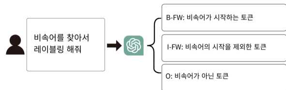
Fig. 2. Labeling Prompt
