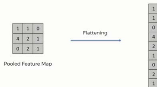
Fig.4: Flattening of max pooled matrix
