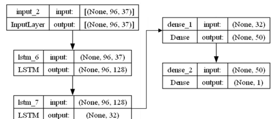
Fig. 11. Structure of LSTM Model(Feature Extraction)
