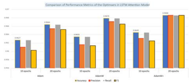
Fig 3 LSTM ATT Model Performance Metrics comparison of 3 Optimizer
