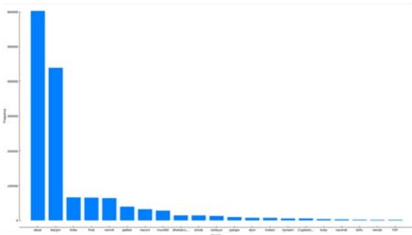
Fig 2 DGA Dataset Visual Breakdown alongwith Alexa being legitimate Dataset
