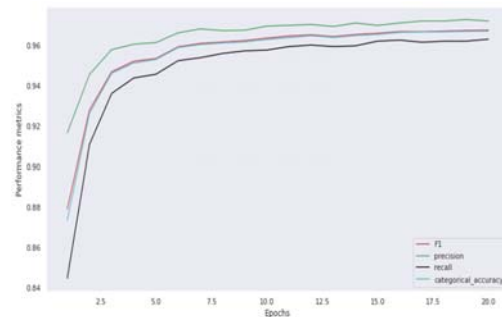
a. LSTM Attention with Adam
