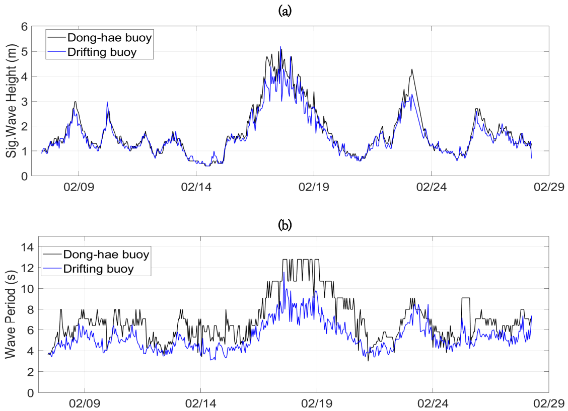
Fig. 4. Time series of (a) significant wave height and (b) wave period from Dong-Hae ocean data buoy and drifting buoy.
