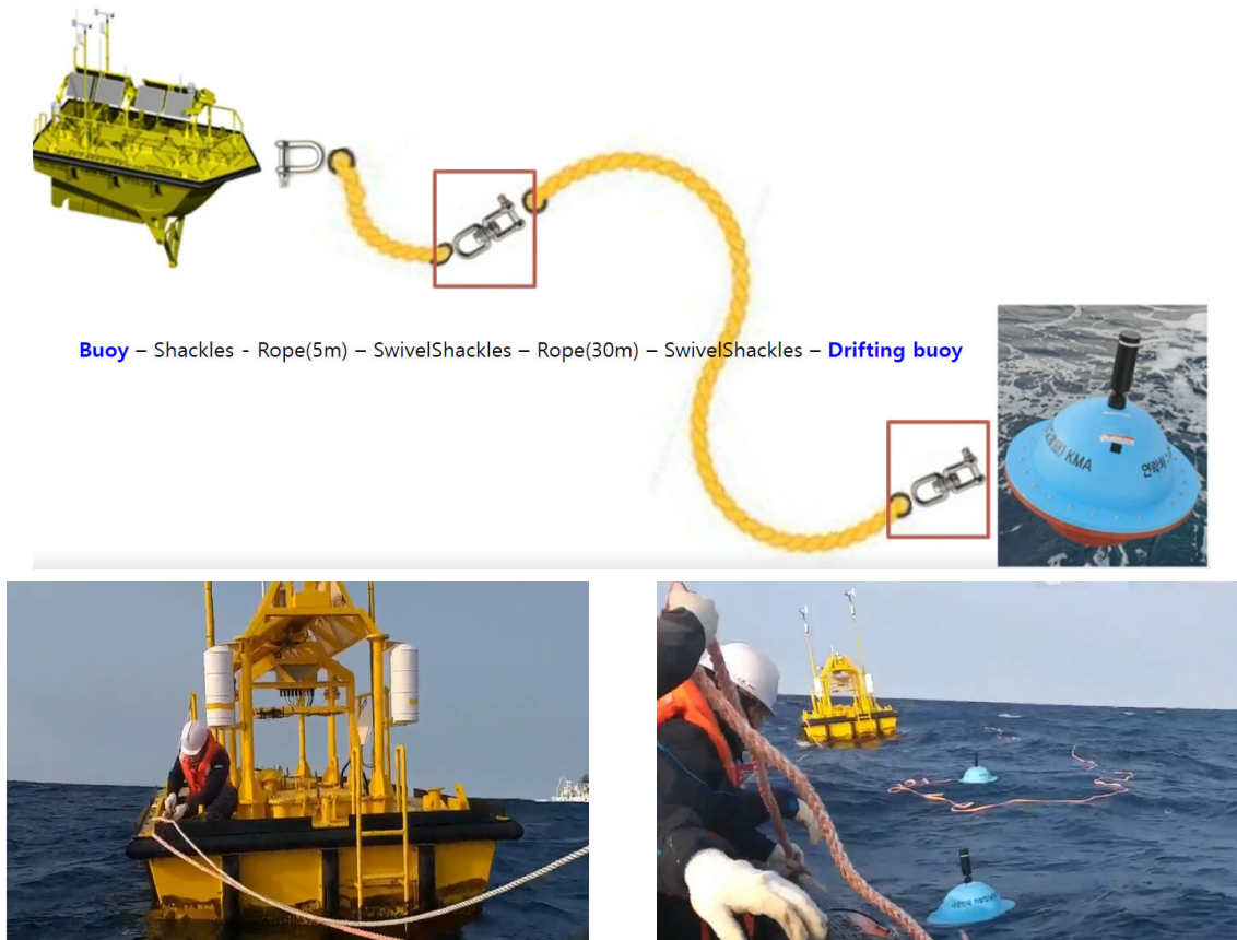
Fig. 2. Design of experiment for analyzing the characteristics of wave observed from ocean data buoy and drifting buoy.
