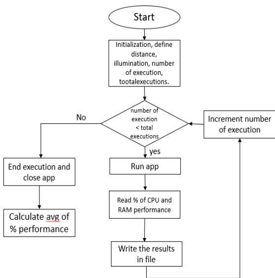
Figure2: Methodology workflow.
