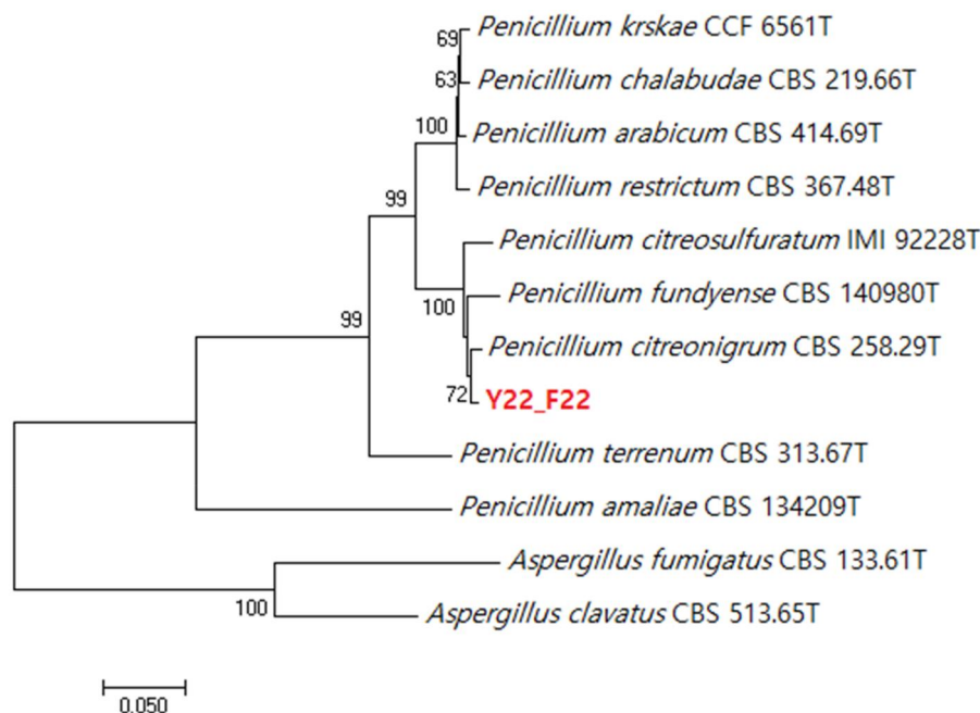
Figure 3. Phylogenetic tree based on maximum likelihood analysis of the combined ITS, BenA , CaM , and RPB2 dataset for species classified in the Penicillium section. Aspergillus fumigatus and Asp. clavatus were included as an outgroup. Bootstrap analysis was performed with 1,000 replications. Bootstrap support values of \geq 60\% are indicated at the nodes. The bar indicates the number of substitutions per position. T indicates the type strains of the species. Bar indicates 0.05 substitutions per nucleotide position. The isolate Y22_F22 is marked in red.
