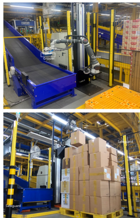
[Fig. 3] Post office collaboration robot parcel depalletized system
