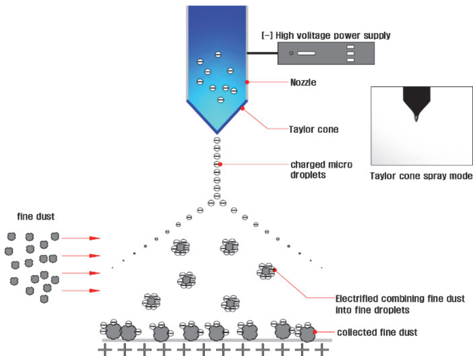
Fig. 1. Schematic diagram of electro-spray method.
