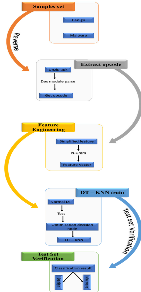
Figure 2: Illustrates the proposed hybrid model for android malware detection by a combination of the decision tree along with the KNN technique. Our suggested developed hybrid model is segregated into the five diverse segments which are sample set and extract opcode along with the features engineering as well as decision tree-KNN and the last one is test set verification.
