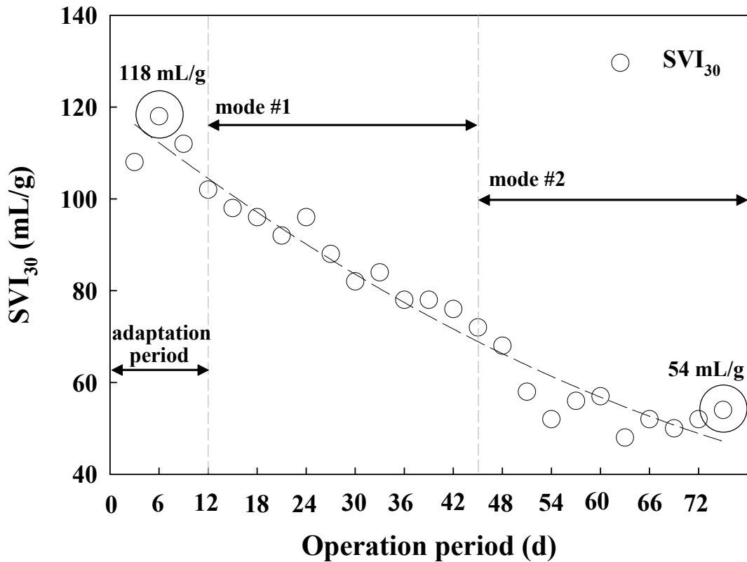
Fig. 5. Results of SVI 30 value during the operation period.
