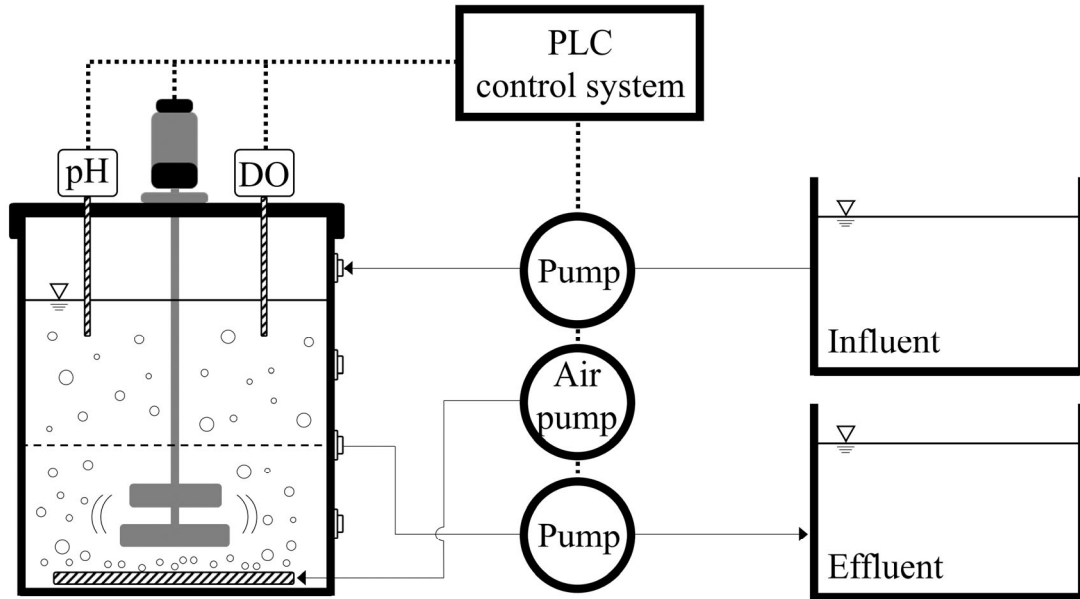
Fig. 1. Schematic diagram of lab. scale reactor.
