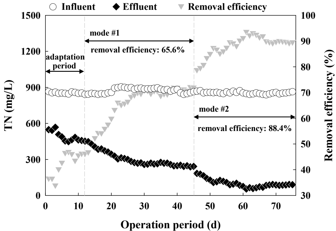
Fig. 3. Results of TN concentration during the operation period.
