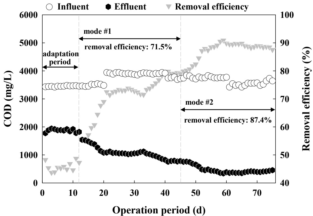
Fig. 2. Results of COD concentration during the operation period.
