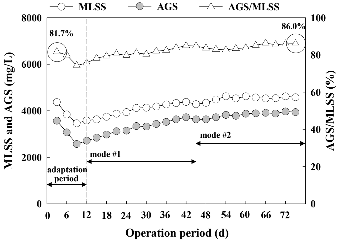
Fig. 4. Results of MLSS, AGS concentration and AGS/MLSS ratio during the operation period.
