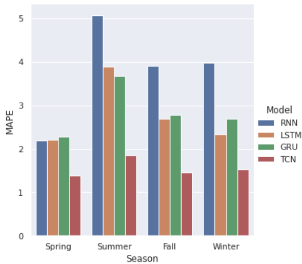
Fig. 10. MAPE Comparison by Season
