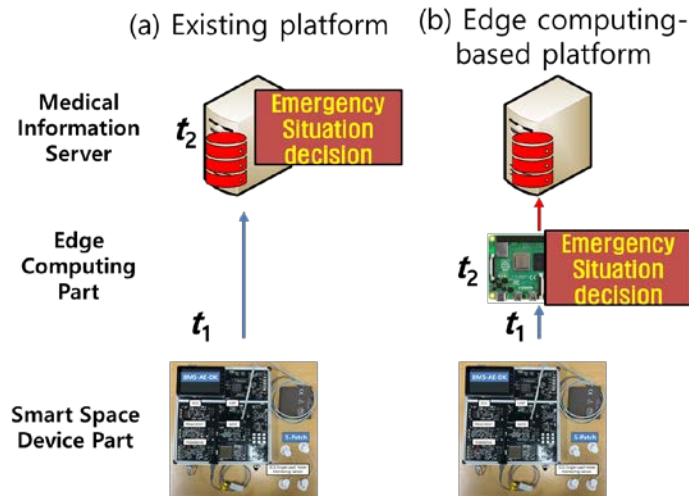
Fig. 5. Test bed for comparison of transmission delay of two platforms. (a) Existing medical information platform without edge computing; (b) Edge computing-based medical information platform.
