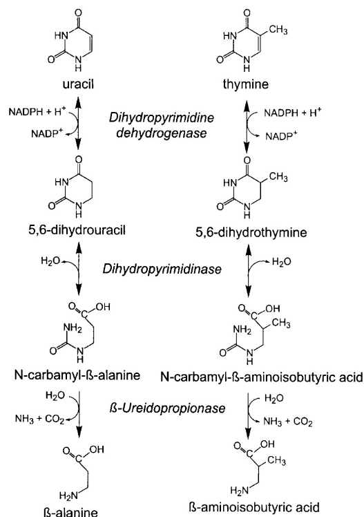
Fig. 2. Catabolic pathway of the pyrimidines uracil and thymine [6].
