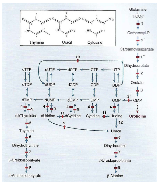
Fig. 1. Pyrimidine metabolism pathways. CMP, cytidine monophosphate; OMP, orotidine monophosphate; dTMP, deoxythymidine monophosphate; UMP, uridine monophosphate. 1, Carbamoylphosphate synthetase II; 1', Aspartate transcarbamylase; 1'', Dihydroorotase (1, 1', and 1'' form a carbamoylphosphate synthetase-aspartate transcarbamylase-dihydroorotase trifunctional protein); 2, Dihydroorotate Dehydrogenase (DHODH); 3, Orotate phosphoribosyltransferase; 3', Orotidine monophosphate decarboxylase (3 and 3' form UMPS); 4, Cytosolic 5'-nucleotidase 3A; 5, Thymidine phosphorylase (TP); 6, Dihydropyrimidine dehydrogenase (DPD); 7, Dihydropyrimidinase (DHP); 8, \beta -ureidopropionase (UP); 9, Thymidine kinase (TK); 10, Ribonucleotide-diphosphate reductase (RRM2B); 11, Cytidine deaminase; 12, Uridine phosphorylase. Deficient enzymes are indicated by red solid bars across the arrows; overactive enzymes are indicated by double red arrows. A red star indicates another causal mechanism. Unusual metabolites consecutive to enzymatic blocks are highlighted in red [4].
