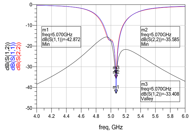
Fig. 9: Simulated S parameters with DGS.
