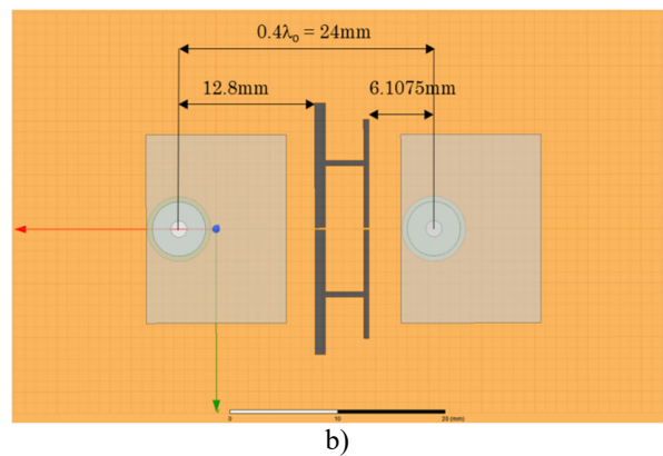
Fig. 6: a) Proposed DGS design structure, b) Array of two collinearly arranged patch antenna elements with carved \mu shaped DGS
