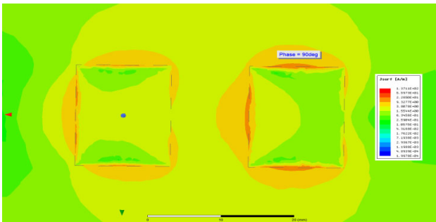
Fig. 7: A screen shot of Surface current distribution without DGS at 90° phase during animation.
