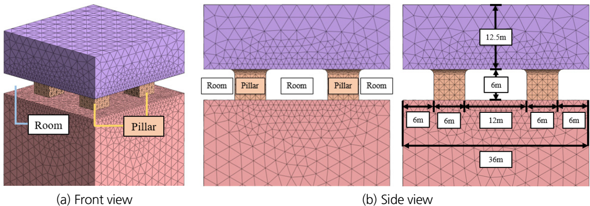
Fig. 2. FEM model mesh geometry
