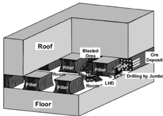
Fig. 1. Room-and-pillar mining (Okubo and Yamatomi, 2009)
