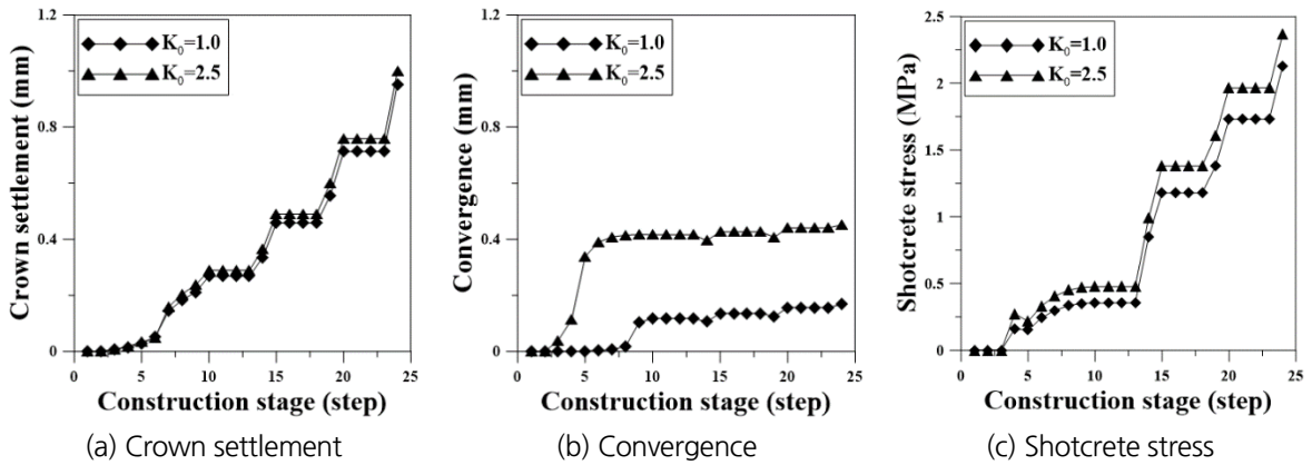
Fig. 5. Result of numerical analysis (Type-1)
