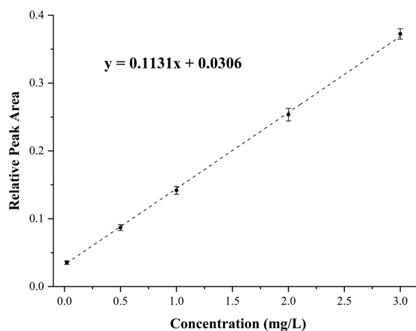
Figure 3. Calibration curve of methyl 2-aminobenzoate for quantitative analysis of the developed RM. The curve was constructed at five different concentrations, i.e., 0.02, 0.5, 1, 2, and 3 mg/L with the addition of the methyl N-methyl-2-aminobenzoate, i.e., 1 mg/L as an internal standard.
