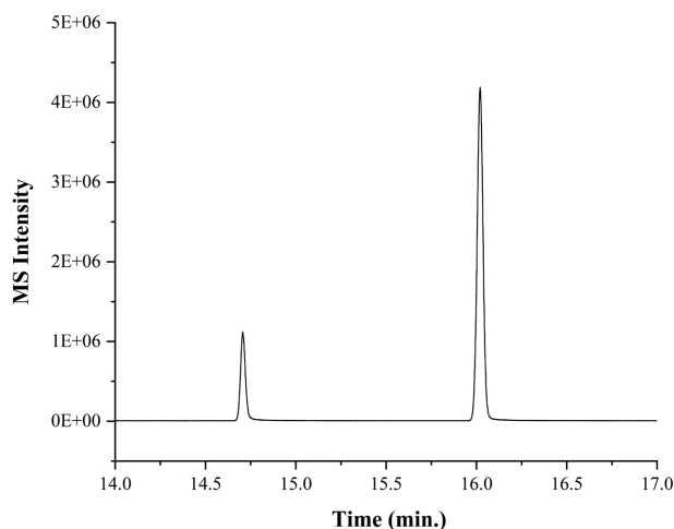
Figure 2. GC-MS chromatogram of the 10-fold diluted RM for methyl 2-aminobenzoate at m/z 119.0 and 92.0, and for methyl N-methyl-2-aminobenzoate at m/z 165.0 and 105.0. The peaks corresponding to methyl 2-aminobenzoate and methyl N-methyl-2-aminobenzoate were observed at 14.70 min and 16.08 min, respectively.
