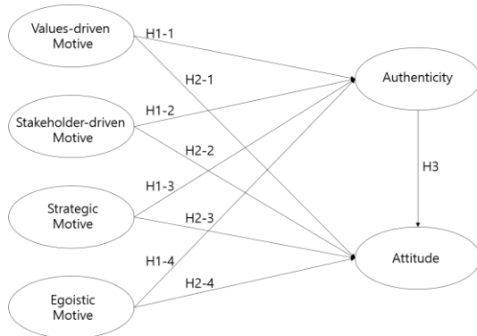
Figure 1: Proposed Model
