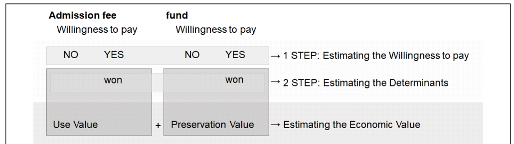
Figure 2. Research flow
