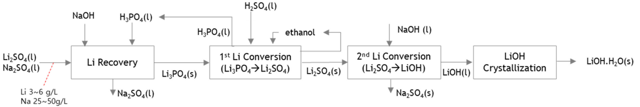
Fig. 3. Precipitation route.
