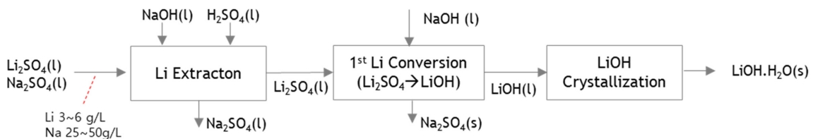
Fig. 4. Extraction route.
