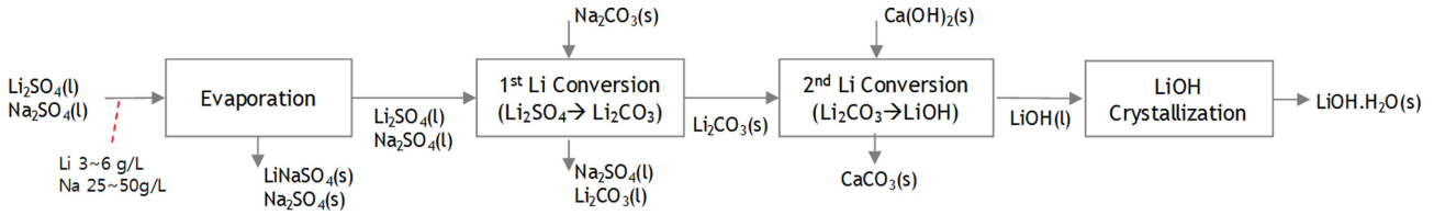
Fig. 2. Evaporation route.
