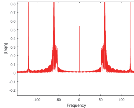
Fig. 9. Spectrum near 60 Hz at checkpoint U4.
