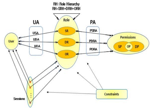
Fig. 6. The Proposed the FA-RBAC
