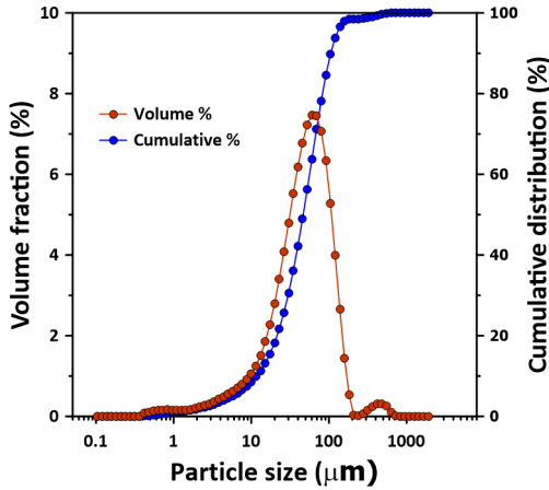
Fig. 2. Particle size distributions of the vanadium concentrations prepared from milled VTM samples used in this study: volume fraction percentage (red circle line) and cumulative distribution percentage (blue circle line).
