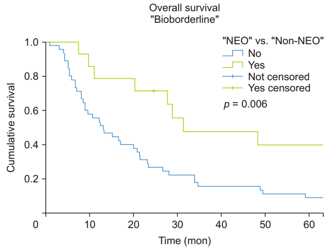
Fig. 3. Overall survival of Bioborderline “NEO vs. Non-NEO”. NEO, Neoadjuvant group; Non-NEO, non-neoadjuvant group.
