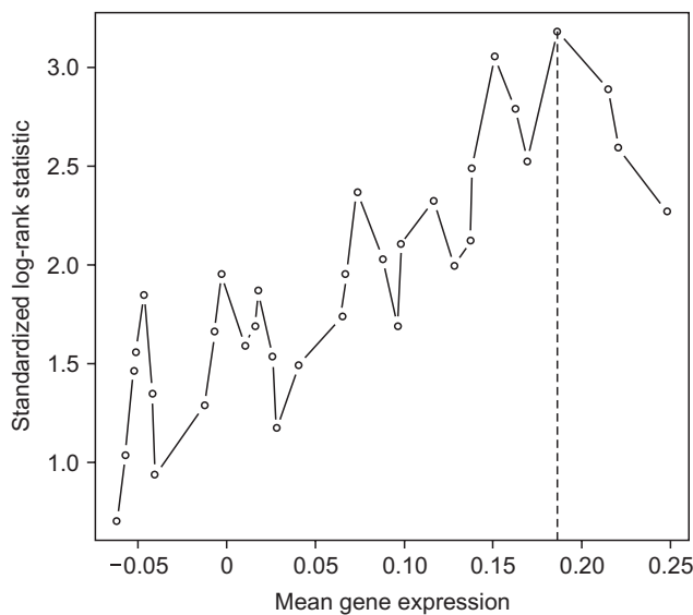
Fig. 3. Standardized log-rank statistic plot.
