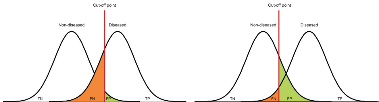
Fig. 1. False positive and false negative according to cut-off point. TN, true negative; FN, false negative; FP, false positive; TP, true positive.
