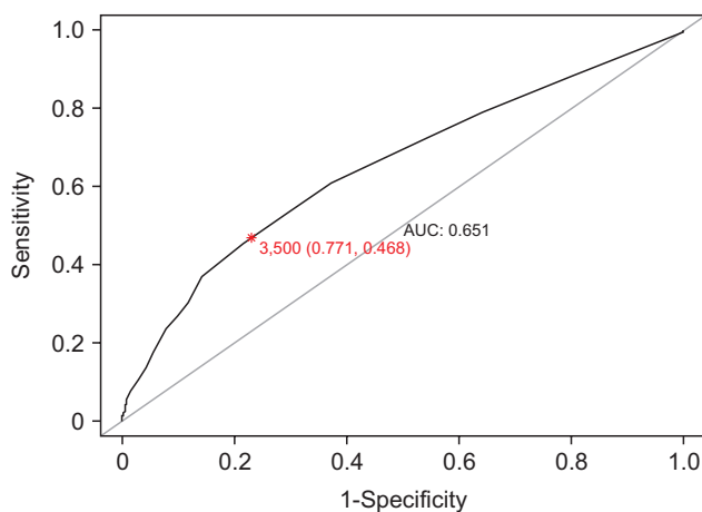
Fig. 2. ROC curve and optimal cut-off point. ROC, receiver operating characteristic; AUC, area under the curve.
