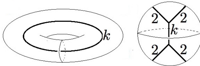
Figure 1: A solid torus V(k) and Conway ball B(k)
