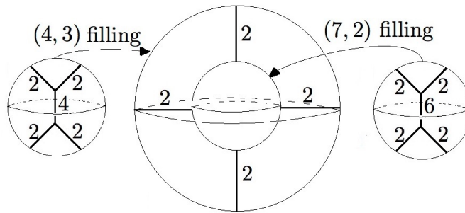
Figure 4: Full quotient space
