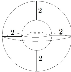
Figure 3: Quotient space (S^1 \times A)/Dih(\mathbb{Z}_6 \times \mathbb{Z}_{12})
