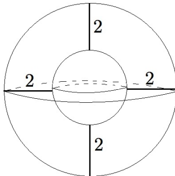
Figure 2: Quotient under the action of Example 6.6
