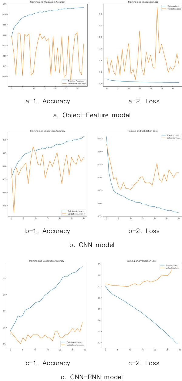
Fig. 11. Training / testing accuracies and losses
