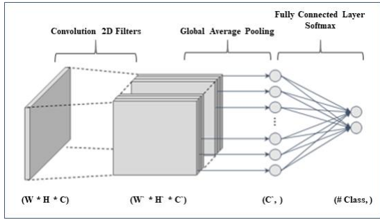
Fig. 5. CNN+FCL based classifier
