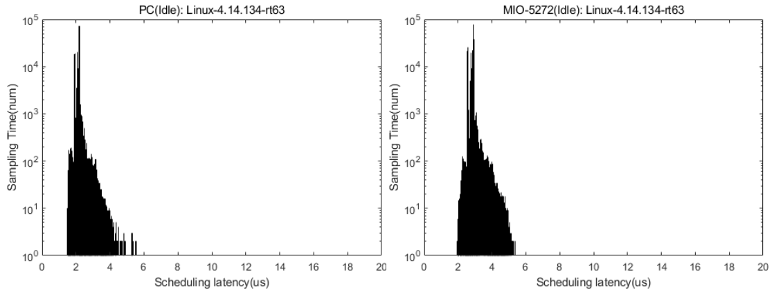
Figure 3. Histogram of scheduling latency in RT-preempt (Idle)
