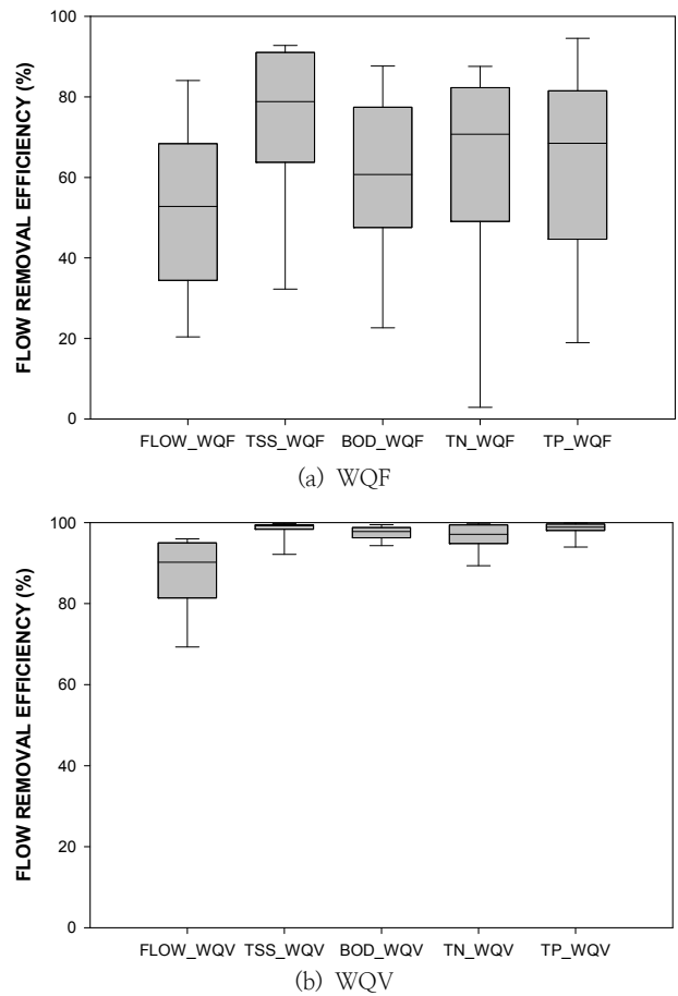
Fig. 4. Comparison of removal efficiency (Flow and pollutants) according to design Factor
