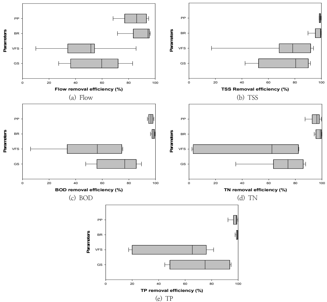
Fig. 3. Flow and pollutants removal efficiency of monitored LID facilities
