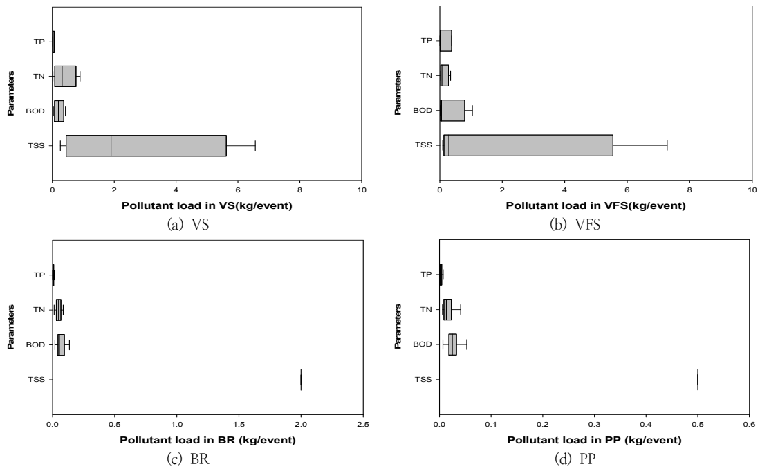
Fig. 2. Inflow pollutants load of monitored LID facilities
