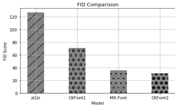
Fig. 18. FID Score Comparison by Models
