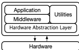
Fig. 1. STM32 firmware architecture
