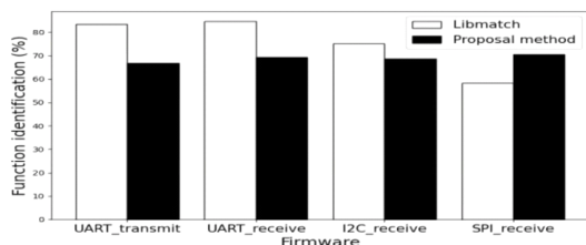
Fig. 3. HAL function identification rate
