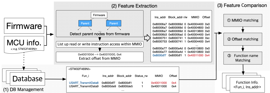
Fig. 2. Pseudo-HAL identification system design
