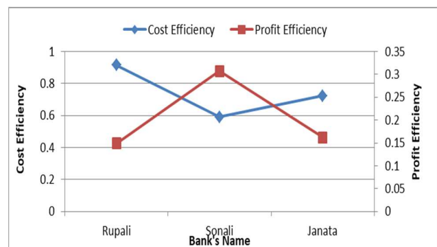
Figure 2: Yearly average cost and profit efficiency of SOCBs with DEA
