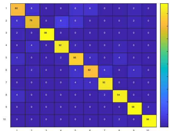
Fig. 10. Confusion matrix of pig identification based on MLDDN by SVM with linear kernel function.
