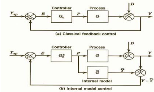
Fig. 4 Basic Block diagram of Internal Model Controller
