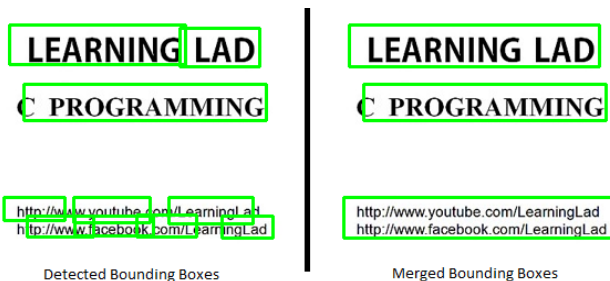
Fig. 4 Merged Bounding Boxes
