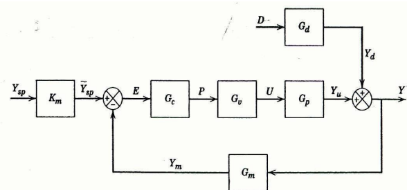
Fig. 3 Block diagram for Direct Synthesis Method
