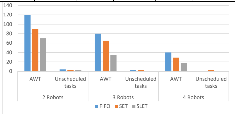
Figure 6. First Experimentation Results using Dataset1, on (2, 3, 4) Robots
