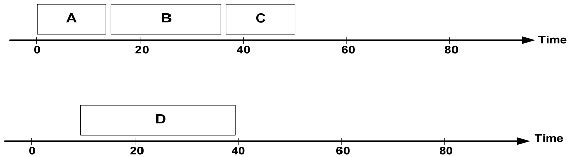
Figure 4. Scheduling problem
