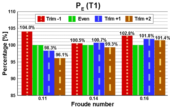
Fig. 6 Relative comparison of effective power at T1
