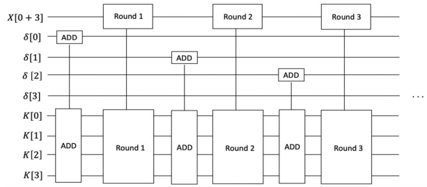
Fig. 5. Previous LEA-128 Quantum Circuit
