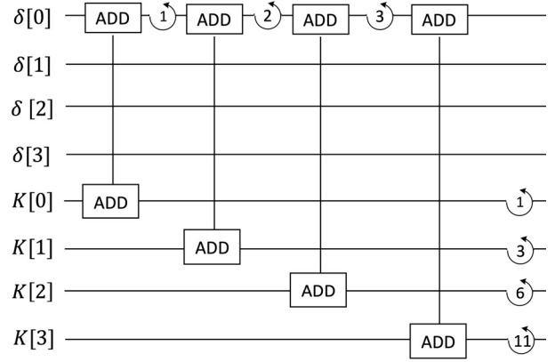
Fig. 4. Previous LEA-128 Key Schedule Quantum Circuit
