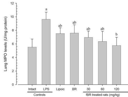
Figure 6. Changes of lung MPO levels.
