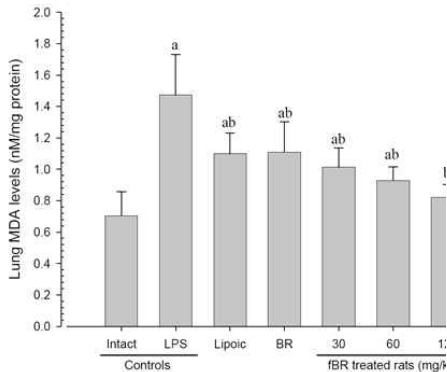
Figure 5. Changes of lung MDA levels.
