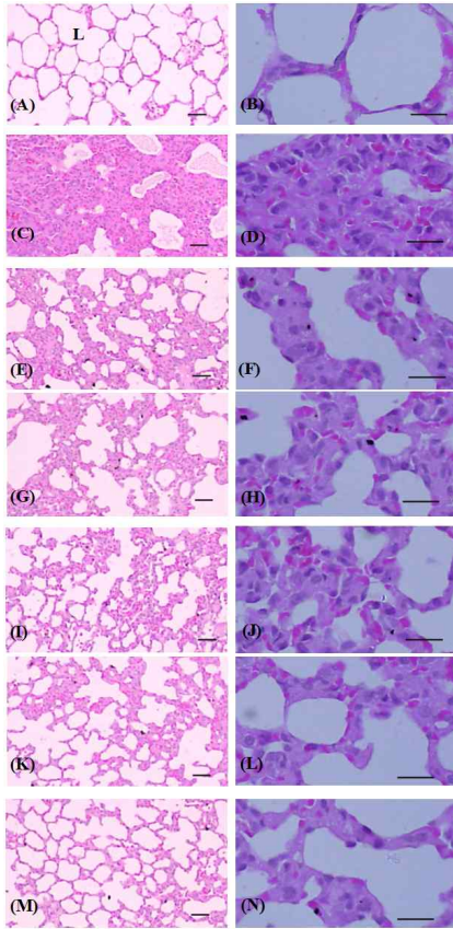
Figure 8. Changes on the lung histopathological profiles
