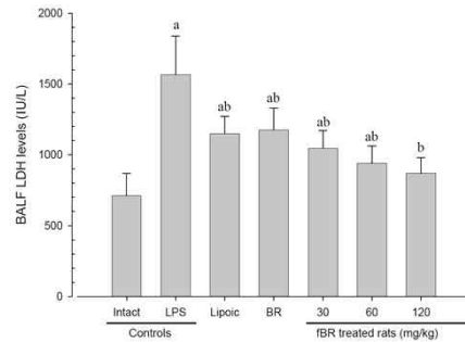
Figure 4. Changes of BALF LDH levels. Note that the BALF LDH levels were significantly ( p<0.01 ) increased in LPS control as compared with intact control. It means lung cellular damages were induced by treatment of LPS. However, these BALF LDH level increases were significantly ( p<0.01 ) inhibited by treatment of \alpha -lipoic acid, BR, fBR 30, 60 and 120mg/kg, respectively; More favorable inhibitions on the BALF LDH increases were detected in fBR 30mg/kg as compared with 60mg/kg of \alpha -lipoic acid and BR treated rats in the present study. Values are expressed mean \pm SD of 8 rats. BALF; brochoalveolar lavgae fluid. LDH; lactate dehydrogenase. LPS; Escherichia coli 0111:B4 lipopolysaccharide (500 \mu g/head). Lipoic; \alpha -lipoic acid 60 mg/kg treated rats. BR; Bupleuri Radix aqueous extracts 60 mg/kg treated rats. fBR; Red-Koji fermented Bupleuri Radix aqueous extract. a p<0.01 as compared with intact control by MW test. b p<0.01 as compared with LPS control by MW test
