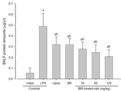
Figure 3. Changes of BALF protein levels. Note that the BALF protein levels were significantly ( p<0.01 ) increased in LPS control as compared with intact control. However, these BALF protein level increases were significantly ( p<0.01 ) inhibited by treatment of \alpha -lipoic acid, BR, fBR 30, 60 and 120 mg/kg, respectively; More favorable inhibitions on the BALF protein level increases were detected in fBR 30 mg/kg as compared with 60 mg/kg of \alpha -lipoic acid and BR treated rats in the present study. Values are expressed mean \pm SD of 8 rats. BALF; brochoalveolar lavgae fluid. LPS; Escherichia coli 0111:B4 lipopolysaccharide (500 \mu g/head). Lipoic; \alpha -lipoic acid 60 mg/kg treated rats. BR; Bupleuri Radix aqueous extracts 60 mg/kg treated rats. fBR; Red-Koji fermented Bupleuri Radix aqueous extract. a p<0.01 as compared with intact control by LSD test. b p<0.01 as compared with LPS control by LSD test.
