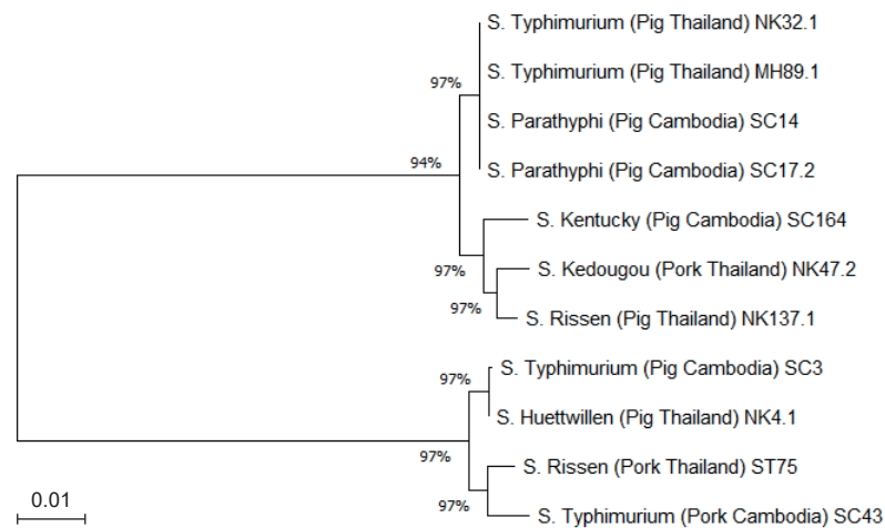
Fig. 1. Phylogenetic tree of the Salmonella isolates (n = 11). Phylogenetic analysis was based on the alignment of the three multi-locus sequence typing genes ( manB , mdh , and fimA ) sequenced. The sequence was aligned by the MUSCLE options in MEGA-X, and a phylogenetic tree was constructed using the neighbor-joining method. The tree was drawn to scale, with branch lengths in the same units as those of the evolutionary distances used to infer the phylogenetic tree.
