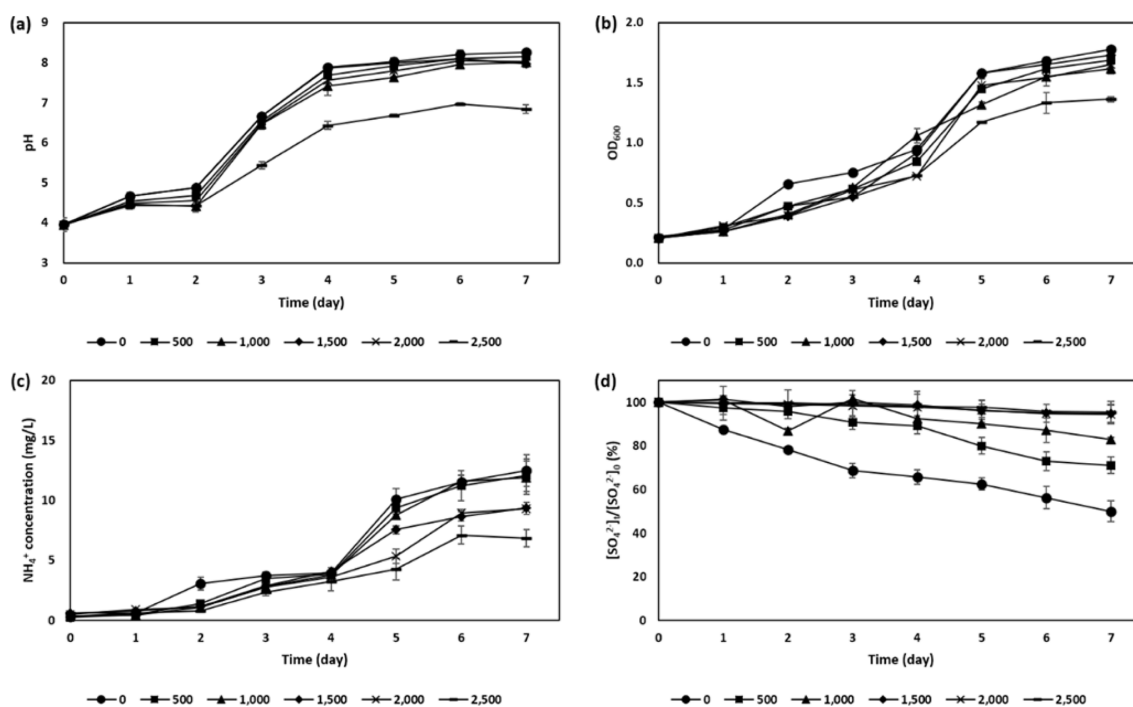
Fig. 1. Temporal variations in (a) pH, (b) microbial density as of OD 600 , (c) NH 4 + concentration, and (d) the percentage of SO 4 2- concentration compared to the initial dose in LB medium in response to different AMD doses from 0 to 2,500 mg SO 4 2- /L.
