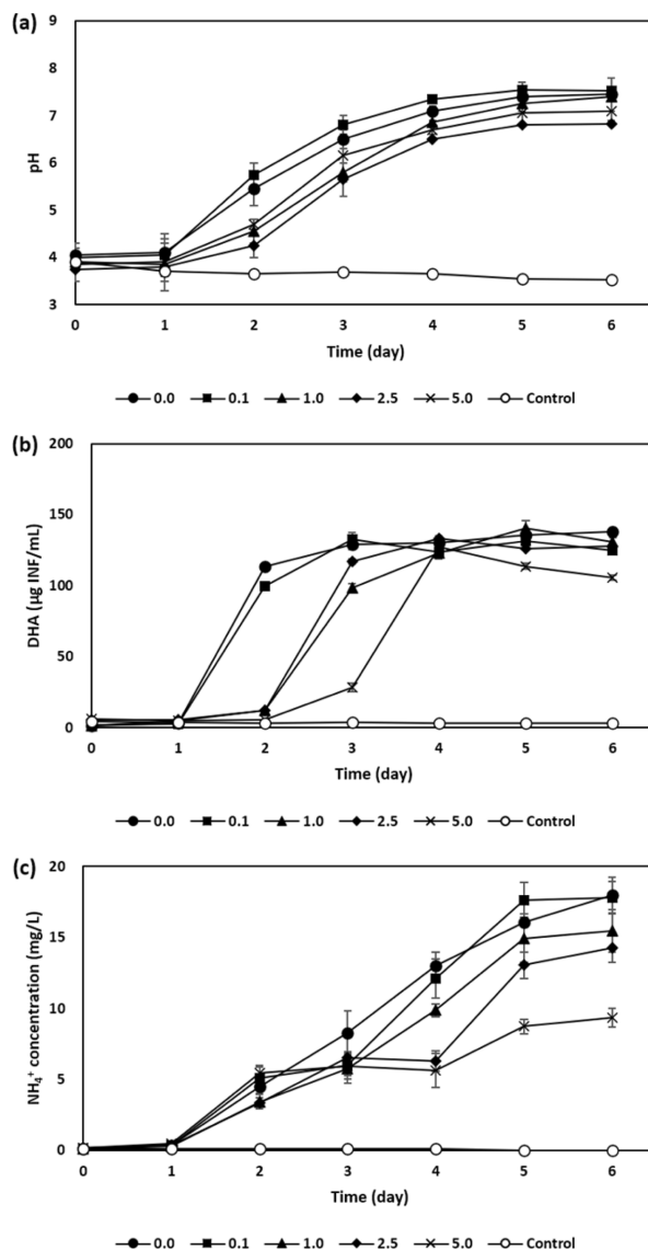
Fig. 3. Comparison of resulting (a) pH, (b) dehydrogenase activity, and (c) NH 4 + concentration of soil slurry containing different amount of sphagnum peat of 0, 0.1, 1, 2.5, and 5 g in an acidic mine soil slurry for 6 days of incubation.
