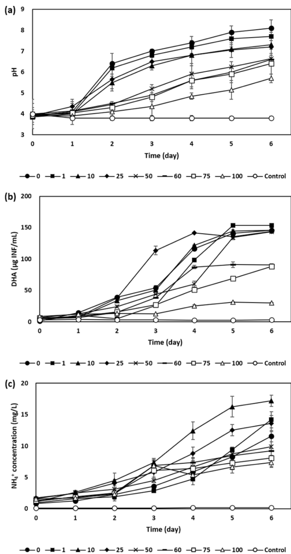
Fig. 2. Variation in (a) pH, (b) dehydrogenase activity, and (c) ammonium (NH 4 + ) concentration of soil slurry containing different amounts of acidic soil (i.e., 0, 1, 10, 25, 50, 60, 75, and 100 g) spiked by AMD for 6 days of incubation.
