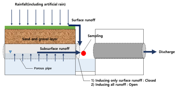
Fig. 2. Facility schematic diagram and sampling point.
