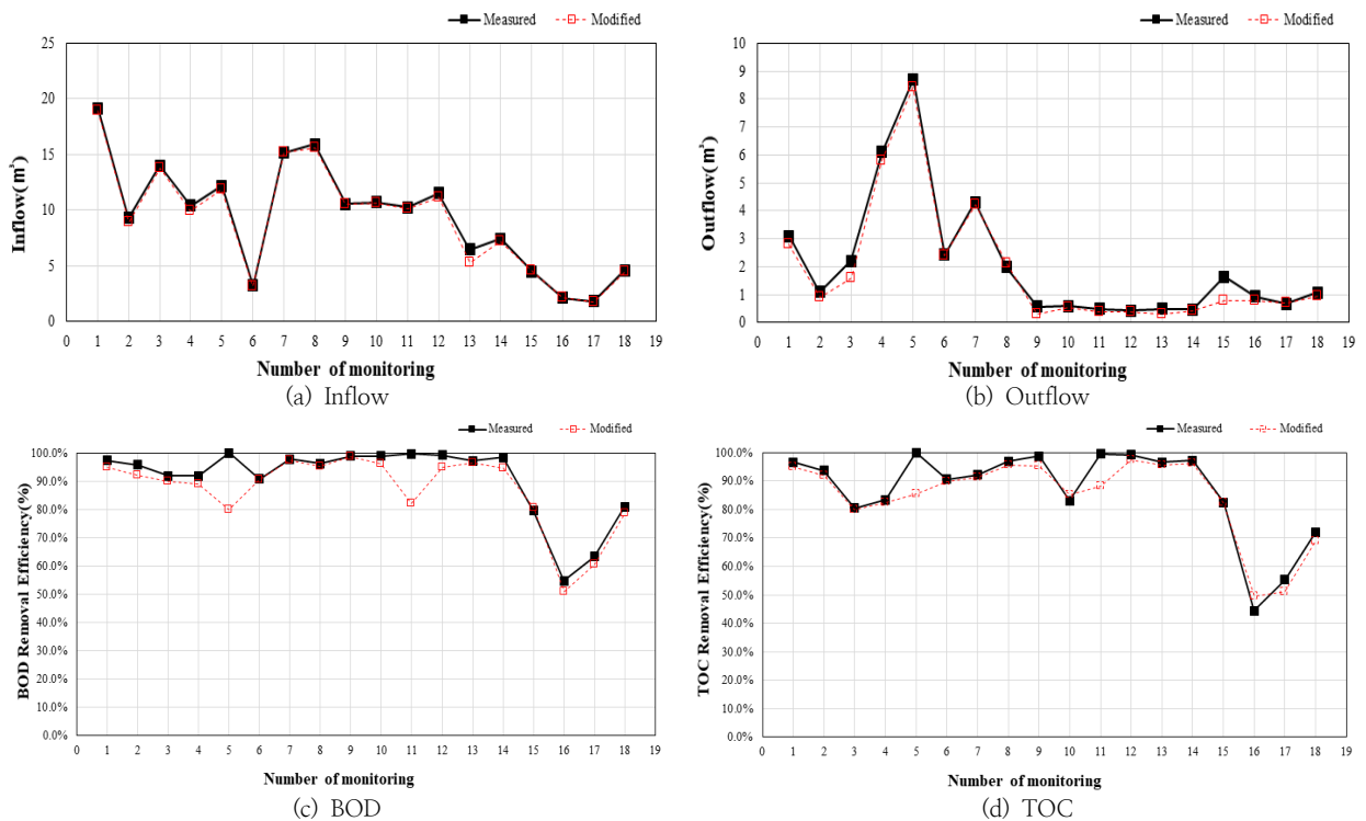
Fig. 3. Simulation results through SWMM model.
