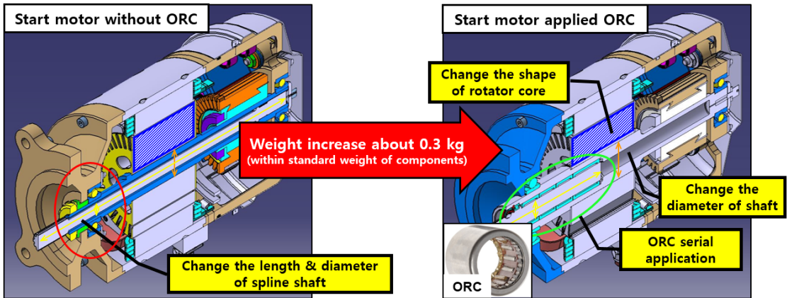
Fig. 6. Configuration of start motor applied ORC
