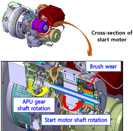
Fig. 3. Start motor cross-section and operating principle
