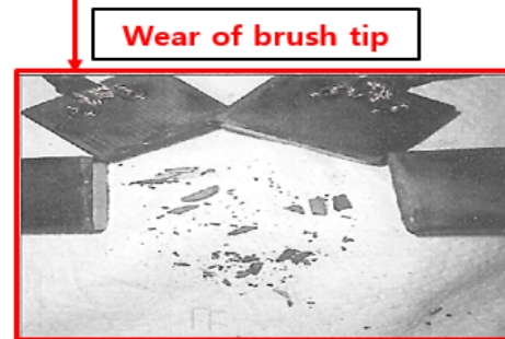
Fig. 2. Configuration of start motor brush & wear defect
