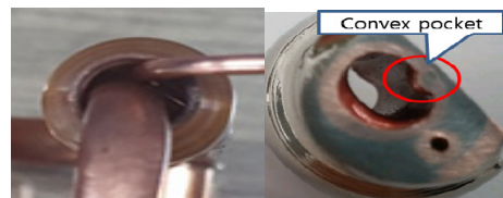
(a) Swaging part insertion structure and welding cutout
