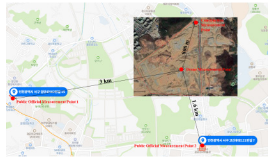
Fig. 2. Distance of drone measurement point
